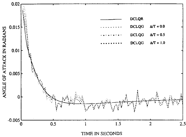
Fig. 2 Transients of angle of attack.
