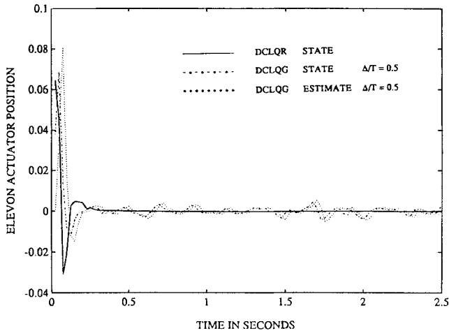
Fig. 4 Transients of elevon actuator position.
