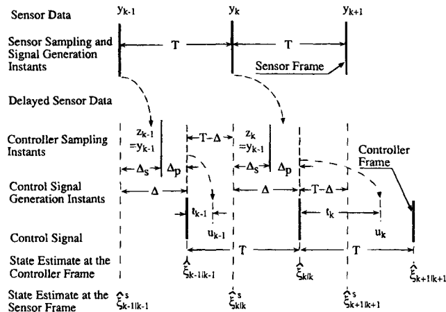
Fig. 1 Illustration of induced delay characteristics.
