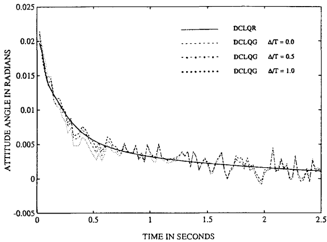
Fig. 3 Transients of attitude angle.
