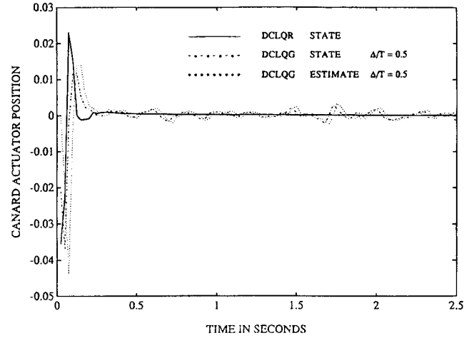
Fig. 5 Transients of canard actuator position.
